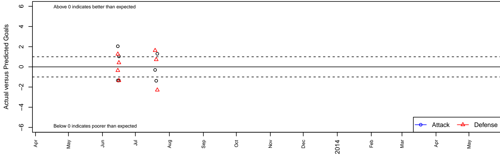
TSS Academy Datillo B98 Dots are actual minus expected GF (blue circles) and GA (red triangles). Blue line is smoothed change in attack strength. Red is smoothed change in defense strength.
